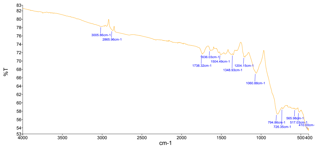
Fig. 3. FTIR test results on SiC impregnated kevlar.
